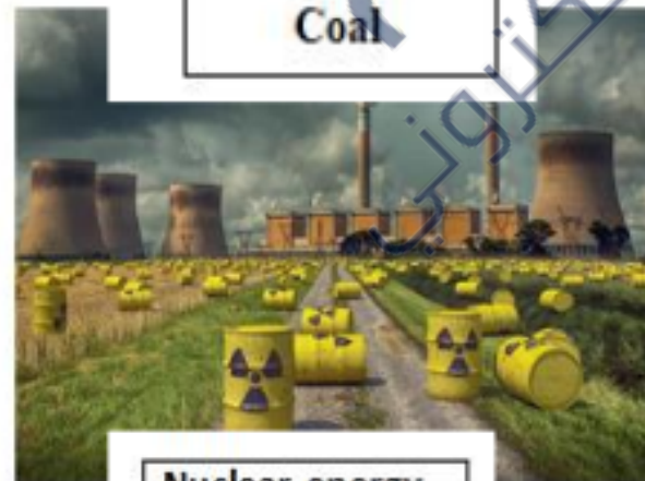
Nuclear energy
